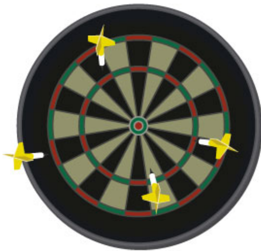
Low Accuracy; Low Precision
