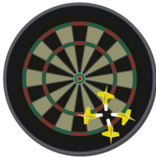
Low Accuracy; High Precision
